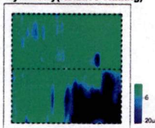
Asymmetry(Relative Thinning)
